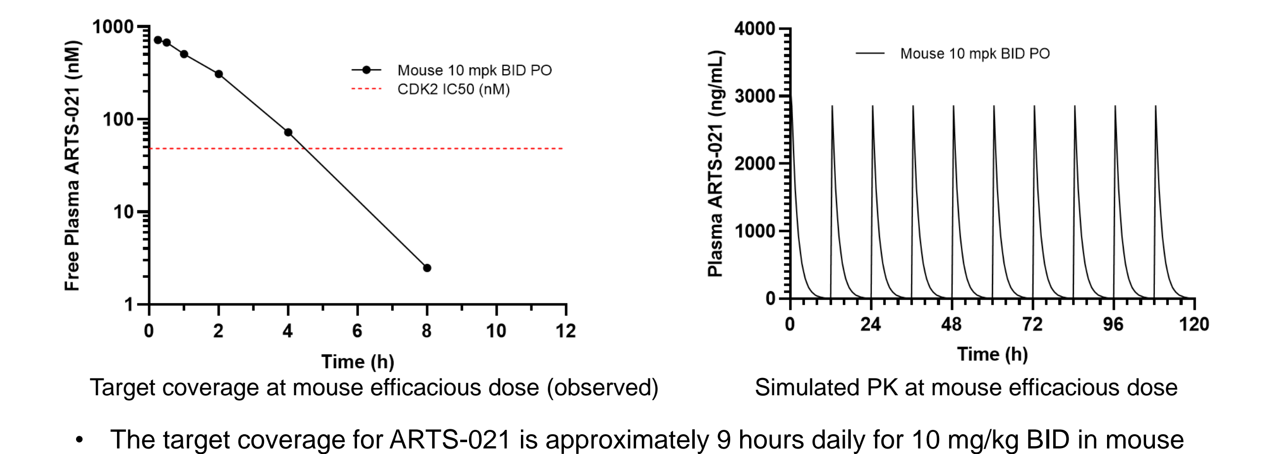
Figure 8. ARTS-021 Mouse PK at efficacious dose of 10 mg/kg BID
